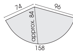
Stool, semi-circular, right 530R
