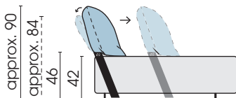
Side view (type 49M)
