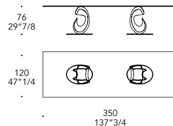
Rectangular 350
