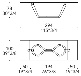
Rectangular 194-294
