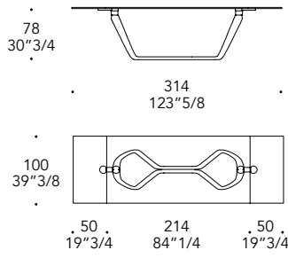
Rectangular 214-314
