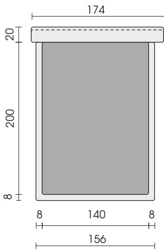
Bed 140 cm B14
