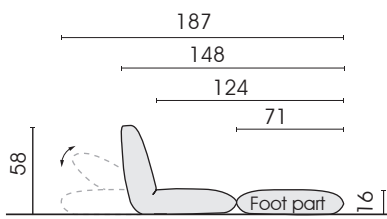
Side view (TYPE 596L)
