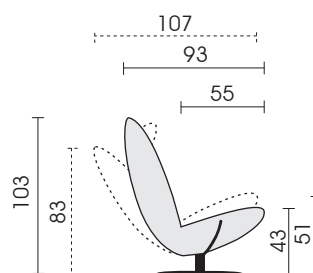
Side view base plate (type 140)
