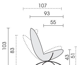
Side view cross frame (type 140)
