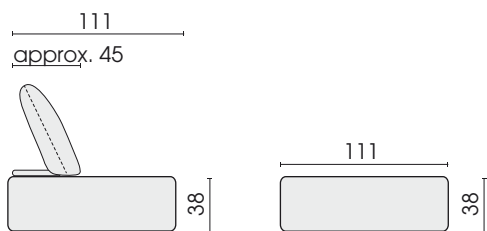
Side view seat element, deep (with back type 611)
