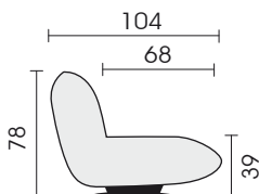
Side view (type 139)
